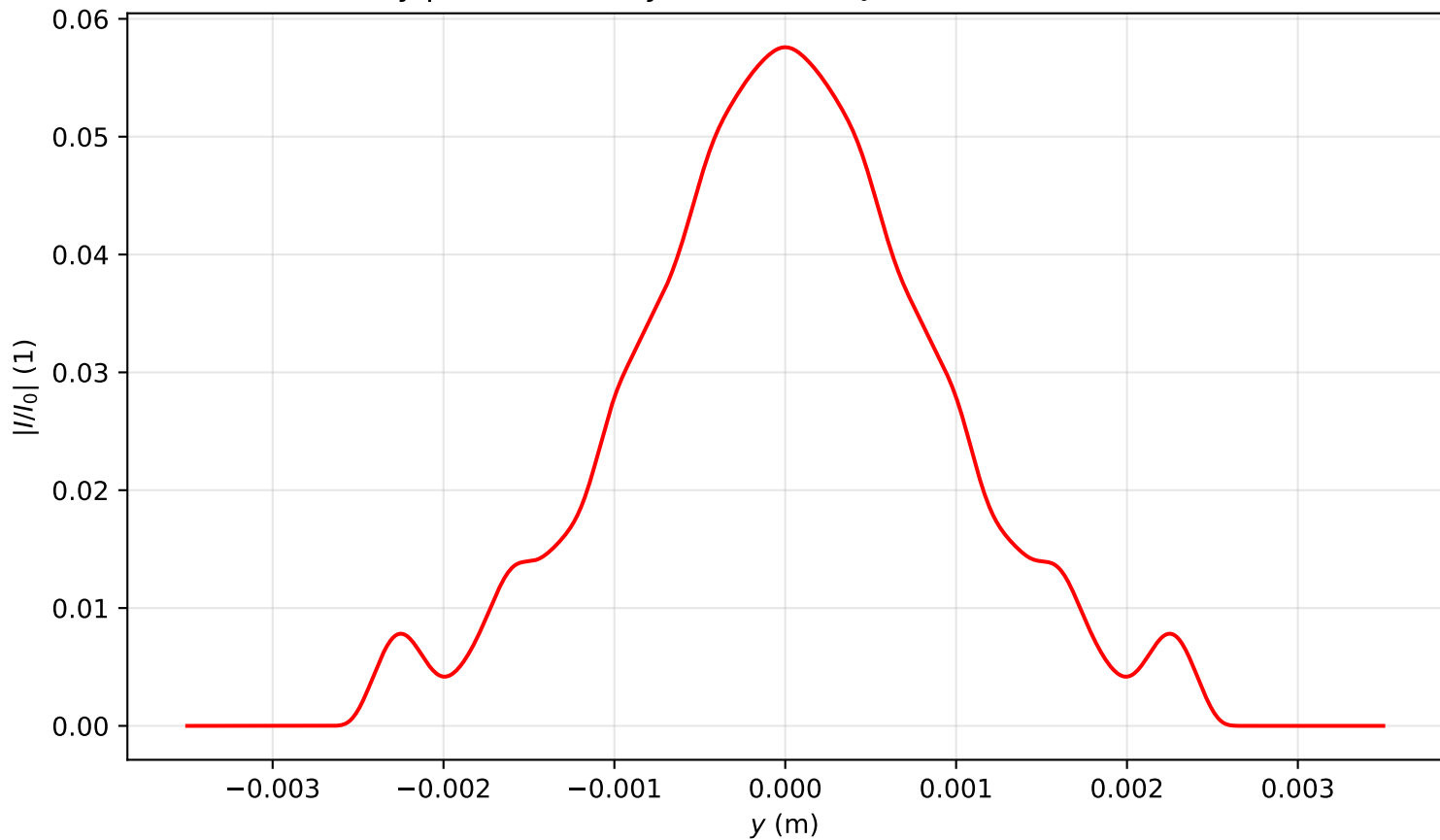
Intensity profile I(x=0, y, z=3.981)/I_0 , P_{in}=2.0P_{cr} , artificial time
